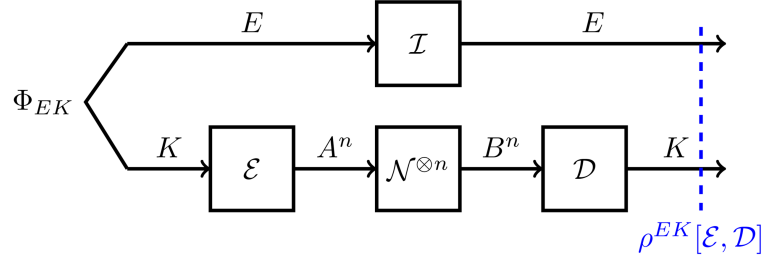
Figure 3 (Color online) Coding scheme for entanglement transmission over n uses of a channel \mathcal{N} \in \text{CPTP}(A \rightarrow B) . The systems E and K are isomorphic. The encoder \mathcal{E} \in \text{CPTP}(K \rightarrow A^n) encodes the part K of the maximally entangled state \Phi_{EK} into the channel input systems. Later, the decoder \mathcal{D} \in \text{CPTP}(B^n \rightarrow K) recovers the state from the channel output systems. The map \mathcal{I} \in \text{CPTP}(E \rightarrow E) is the identity map. The final state after the coding strategy is denoted as \rho_{EK}[\mathcal{E}, \mathcal{D}] and the performance of the code is quantified using the fidelity F(\Phi_{EK}, \rho_{EK}[\mathcal{E}, \mathcal{D}]) .
