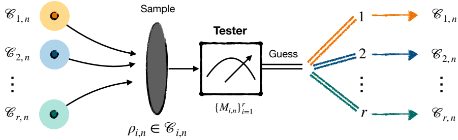
Figure 1: Quantum hypothesis testing for multiple sets of quantum states \mathcal{C}_{1,n}, \dots, \mathcal{C}_{r,n} .
