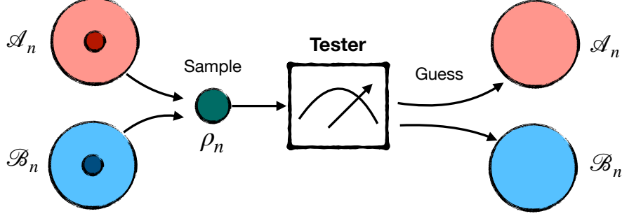
Figure 1: An illustration of the quantum hypothesis testing between two sets of quantum states \mathcal{A}_n and \mathcal{B}_n . A tester draws samples from the sets and performs quantum measurement to determine which class the sample belongs to. The null hypothesis is that the sample is from \mathcal{A}_n , which typically represents the bad case, and the alternative hypothesis is that the sample is from \mathcal{B}_n .
