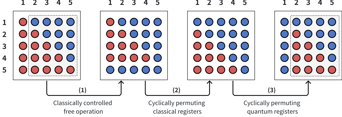
Figure 2: An illustration for the steps of the procedure used to prove Theorem 3, for the case where n = 15 , m = 5 , and therefore k = 3 . Each dot represents a quantum state on the system S^3 . Red dots correspond to groups of states \zeta = \rho^{\otimes 3} \in \mathcal{D}(S^3) , while blue dots represent embedded states \hat{\sigma} = \sigma \otimes \pi^{\otimes 2} \in \mathcal{D}(S^3) that match the system of \zeta . The overall quantum state is a mixture of rows, each labeled with a classical register. In the first step, a classically controlled free operation is applied, transforming the last row from \zeta^{\otimes 5} = \rho^{\otimes 15} to \hat{\sigma}^{\otimes 5} . The second step involves cyclically permuting the classical registers (i.e., the rows of dots), and the third step involves cyclically permuting the quantum registers (i.e., the columns of dots). The dashed boxes highlight the catalyst state, showing that it remains unchanged before and after the transformation.
