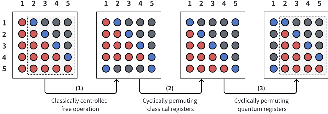
Figure 3: An illustration for the steps of the procedure used to prove Theorem 7, for the case where n = 5 , m = 2 , and k = 1 . Each dot represents a quantum state on the system T . Red dots correspond to the embedded source state \tilde{\rho} \in \mathcal{D}(T) , while blue dots represent the embedded target state \tilde{\sigma} \in \mathcal{D}(T) . Grey dots represent the embedded free state \tilde{\theta} \in \mathcal{D}(T) , which is orthogonal to \tilde{\sigma} . The overall quantum state is a mixture of rows, each labeled with a classical register. In the first step, a classically controlled free operation is applied, transforming the last row from \tilde{\rho}^{\otimes 5} to \tilde{\sigma}^{\otimes 2} \otimes \tilde{\theta}^{\otimes 3} . The second step involves cyclically permuting the classical registers (i.e., the rows of dots), and the third step involves cyclically permuting the quantum registers (i.e., the columns of dots). The dashed boxes highlight the catalyst state, showing that it remains unchanged before and after the transformation.
