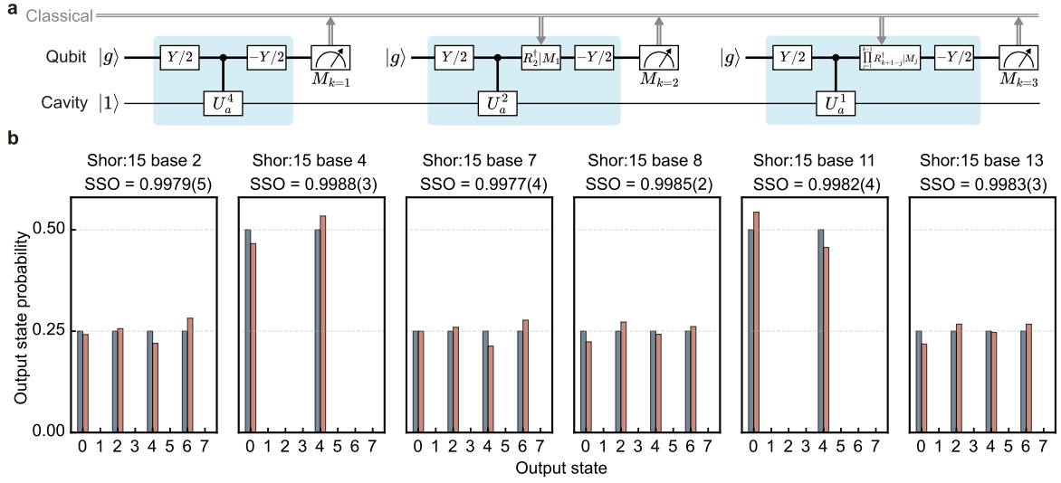
Fig. 4: Experimental realization of DQC for Shor’s algorithm. a DQC sequence for the quantum order-finding subroutine. The cavity is initialized in the Fock state |1\rangle , while the qubit is initialized in |g\rangle and repeatedly measured and reset. The protocol consists of sequential cycles implementing controlled modular exponentiation operations ( U_a^4 , U_a^2 , and U_a^1 ), interleaved with single-qubit rotations and mid-circuit measurements M_k . The first measurement yields a deterministic outcome |g\rangle , and the experiment proceeds from the subsequent cycles. Classically conditioned phase rotations are applied based on prior measurement outcomes. b Measured (red bars) and ideal (blue bars) state probability distributions for coprime bases a \in \{2, 4, 7, 8, 11, 13\} . The SSO between each measured and ideal distribution is calculated and indicated above each panel.
