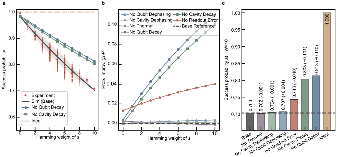
Fig. 8: Numerical simulation of the BV algorithm. a Experimentally measured (red dots) and numerically simulated (solid lines) success probability of the BV algorithm as a function of the Hamming weight (HW) of the hidden bit string s . The base simulation (solid black line) includes all dissipative processes present in the experiment, and the “No qubit decay” and “No cavity decay” denote the simulations that exclude the qubit and cavity decay, respectively. The ideal case corresponds to the simulation with only ideal operations. b Success probability improvements as a function of the HW, obtained by comparing the simulated success probability with and without considering the specific error sources. c Simulated success probabilities with removing the specific error channels at HW = 10. The values of the bar heights are indicated, with the values in parentheses denoting the corresponding success probability improvement \Delta P . Qubit and cavity decay are the dominant error sources, contributing infidelities of about 0.11 and 0.10, respectively.
