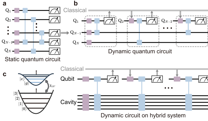
Fig. 1: Schematic illustration of DQCs on a hybrid superconducting qubit-cavity processor. a Conventional static quantum circuit with N qubits. b Dynamic circuits: the upper qubit is measured, reset, and reused sequentially with real-time feed-forward. c Implementation of DQCs on a hybrid superconducting qubit-cavity system, where a transmon qubit is dispersively coupled to a long-lived cavity. The cavity's multi-level Hilbert space serves as the computational register and the transmon is repeatedly measured and reused.
