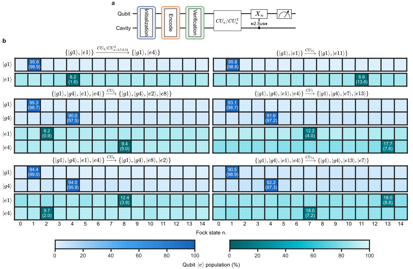
Fig. 7: Characterizing the GRAPE-optimized controlled-unitary operations. a Experimental sequence for evaluating the state mapping performance. After initializing the system in |g, 0\rangle , we encode the system in different input states, apply the optimized controlled-unitary operations, and measure the qubit excited-state populations following an n -photon-number-selective \pi pulse. b Measured qubit excited-state populations with the selective pulse applied on different photon numbers n for the six controlled operations. The left labels denote the input states, and the target mappings are indicated above each matrix. The matrix elements represent the measured qubit excited-state populations after the photon-number-selective \pi pulse, with the values in parentheses obtained from numerical simulations.
