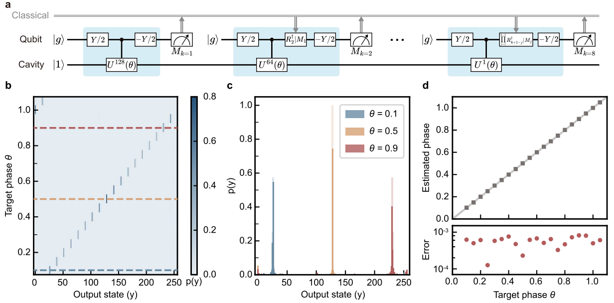
Fig. 3: Experimental realization of DQC for the 8-bit QPE algorithm. a DQC sequence for the QPE algorithm. The cavity is initialized in Fock state |1\rangle , an eigenstate of the unitary operator U = e^{i2\pi\theta a^\dagger a} , while the transmon is initialized in ground state |g\rangle and repeatedly measured and reset. The protocol consists of eight adaptive cycles, each including controlled- U^{2^{8-k}} operations, single-qubit rotations, a mid-circuit measurement M_k , and classically conditioned phase gates implemented via virtual phase rotations. b Measured probability distributions of the binary output states y for target phases \theta \in \{0.1, 0.15, \dots, 1.05\} , obtained from 45,000 repetitions of the experiment for each phase. c Three representative horizontal cuts from b , showing the measured (solid bars) and ideal (shaded bars) probability distributions p(y) for target phases \theta = 0.1, 0.5 , and 0.9 . d Estimated phase \hat{\theta} (top panel) as a function of the target phase \theta , showing good agreement with the ideal prediction (solid line), with the estimation errors shown in the bottom panel. For each phase, the total measurement resources are fixed at R = 200 , and the circuit containing m = 8 measurement rounds is repeated \lfloor R/m \rfloor times. The full dataset of 45,000 circuit repetitions is divided into 1800 independent phase-estimation trials to compute the error bars, which are smaller than the symbol size and thus are not shown.
