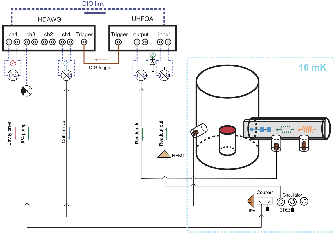
Fig. 5: Measurement setup and experimental device schematic.
