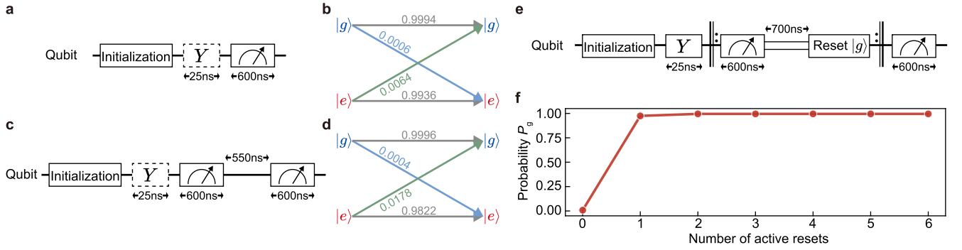
Fig. 6: Characterization of qubit readout and QND fidelity. a Experimental sequence for evaluating the measurement fidelity. b Measured readout fidelities: p_g = 0.9994 and p_e = 0.9936 . c Experimental sequence for extracting the QND fidelity. d Measured QND fidelities: p_{gg} = 0.9996 and p_{ee} = 0.9822 . e Experimental sequence for characterizing the active qubit reset with measurement-based feedback control. f Measured qubit ground-state probability as a function of the number of active resets.
