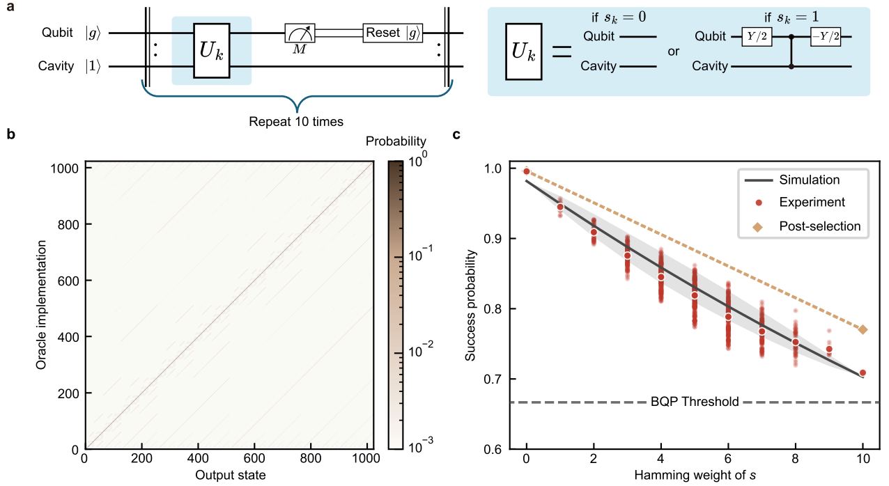
Fig. 2: Experimental realization of DQC for the 10-bit BV algorithm. a DQC sequence for the BV algorithm. The protocol comprises 10 iterative cycles, each corresponding to one bit s_k of the hidden string s . The system is initialized in |g, 1\rangle . Each cycle contains a conditional operation U_k , a mid-circuit measurement ( M ), and a measurement-based qubit reset. The operation U_k is conditioned on s_k : applying a CNOT-type operation if s_k = 1 , while idling if s_k = 0 . b Measured output-state probability distribution for all 2^{10} = 1024 oracle configurations, each obtained from 45,000 repetitions. The correct outputs correspond to the dominant diagonal elements. c Algorithmic success probability versus the Hamming weight (HW) of the hidden string s . Red dots and the black curve denote the experimental and simulated success probabilities, respectively. The success probability ranges from 70.9% (HW = 10) to 99.6% (HW = 0), with an overall average of 82.0%. Post-selecting the cavity in |1\rangle improves the success probability (orange dashed line) by about 6% for HW = 10 and negligibly for HW = 0. All experimental instances exceed the standard 2/3 BQP threshold.
