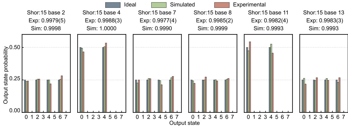
Fig. 10: Measured and simulated probability distributions for Shor's algorithm with coprime bases a \in \{2, 4, 7, 8, 11, 13\} . In each panel, the experimental results (red bars) are compared with numerical simulations that include all identified error sources (green bars), and with the ideal theoretical distributions (blue bars). The corresponding SSO values are displayed above each panel.
