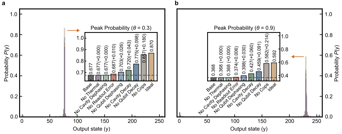
Fig. 9: Error analysis of the QPE experiment. a Measured and simulated probability distributions of the output state y for estimating the target phase \theta = 0.3 . The inset shows the simulated peak probabilities with and without the specific dissipative channels to extract their contributions to the infidelity. The “no cops” result corresponds to the simulation without any collapse operators (retaining only readout infidelity) and agrees well with the ideal theoretical value. The base simulation includes all collapse channels and exhibits good agreement with the experimental peak probability. b Error analysis similar to a but for \theta = 0.9 .
